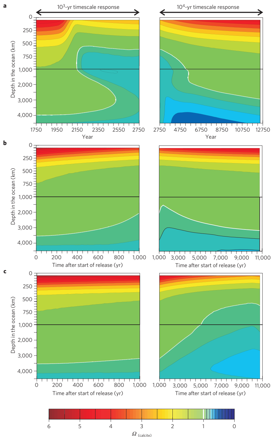
Figure 2 | Anthropogenic and PETM evolution of ocean carbonate saturation in the model. a , Time evolution of ocean \Omega_{(\text{calcite})} (horizontally averaged) under modern boundary conditions and in response to historical CO 2 emissions to 2000 then IS92a CO 2 emissions scenario 14 to 2100, with a linear decline to achieve a cumulative release of 2,180 PgC. b , Time evolution of ocean \Omega_{(\text{calcite})} (horizontally averaged) under late Palaeocene boundary conditions and in response to uniform 2,180 PgC release over 1 kyr. Despite starting slightly more undersaturated ( \Omega < 1.0 ) than modern, the decrease in \Omega at depth is less pronounced, partly a consequence of the higher calcium ion concentration of the Palaeocene ocean. c , Time evolution of ocean \Omega_{(\text{calcite})} (horizontally averaged) under late Palaeocene conditions and in response to uniform 6,840 PgC release over 10 kyr. All three experiments include both climate and deep-sea sedimentary feedbacks.
